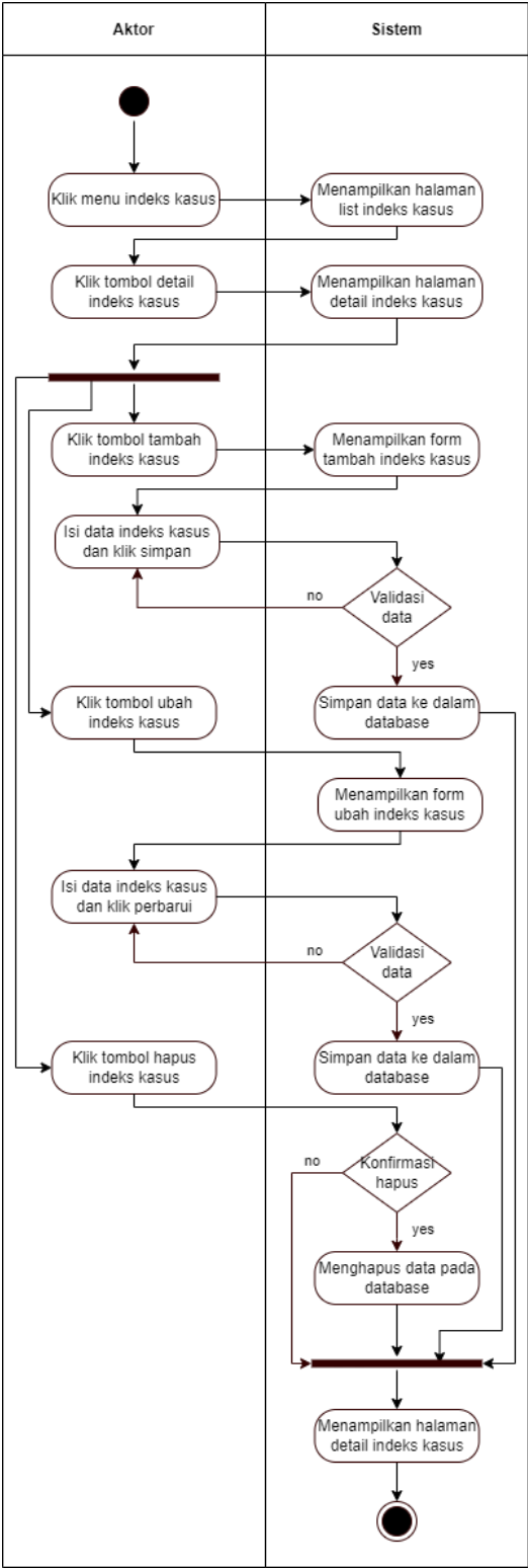
Gambar 6. Activity Diagram kelola indeks kasus
